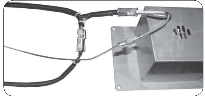
Fig. 21-2 Wire connections
