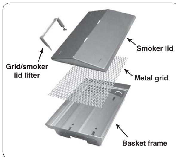
Fig. 30-1 Charcoal/smoker basket items
