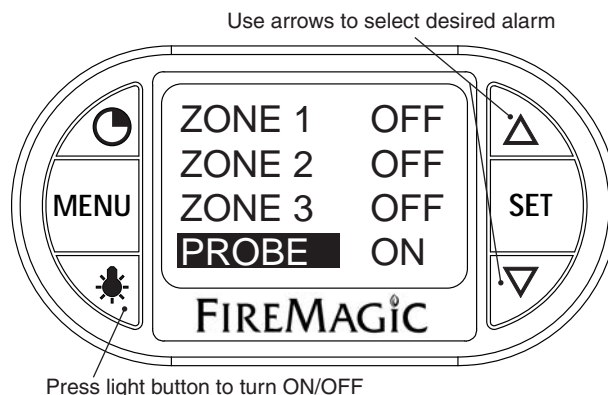
Fig. 27-1 Alarm screen
