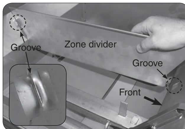
Fig. 19-2 Install zone dividers
