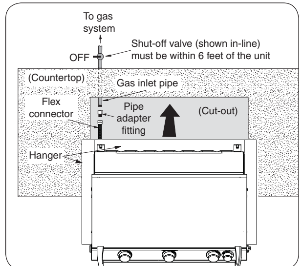
Fig. 18-4 Household propane & natural gas diagram
