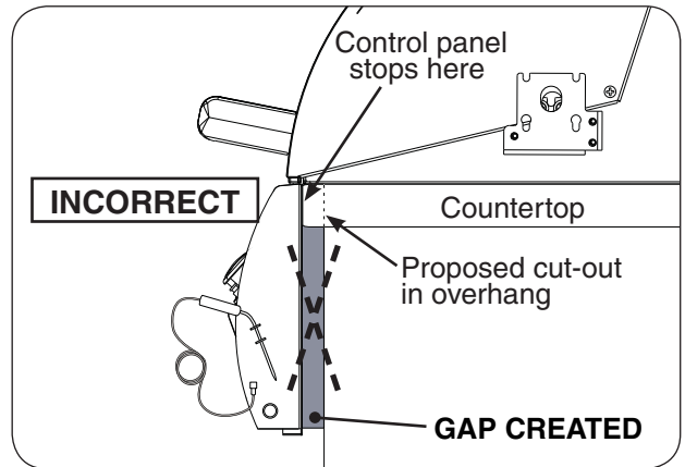
Fig. 18-1 Countertop overhang - incorrect cutout
