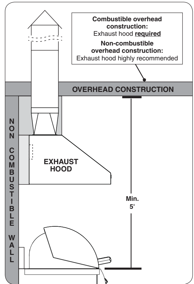
Fig. 11-1 Overhead requirements
