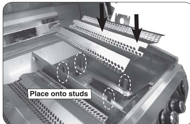
Fig. 19-3 Install flavor grids
