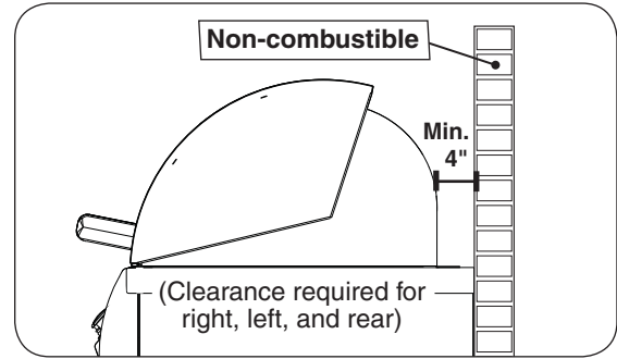
Fig. 12-2 Clearance 'A' Diagram
